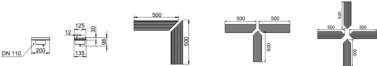
Vertical outlet
